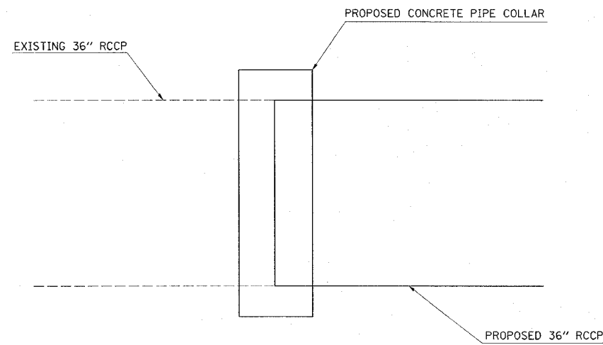
CONCRETE COLLAR TOP VIEW
