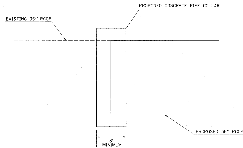
CONCRETE COLLAR SIDE VIEW
