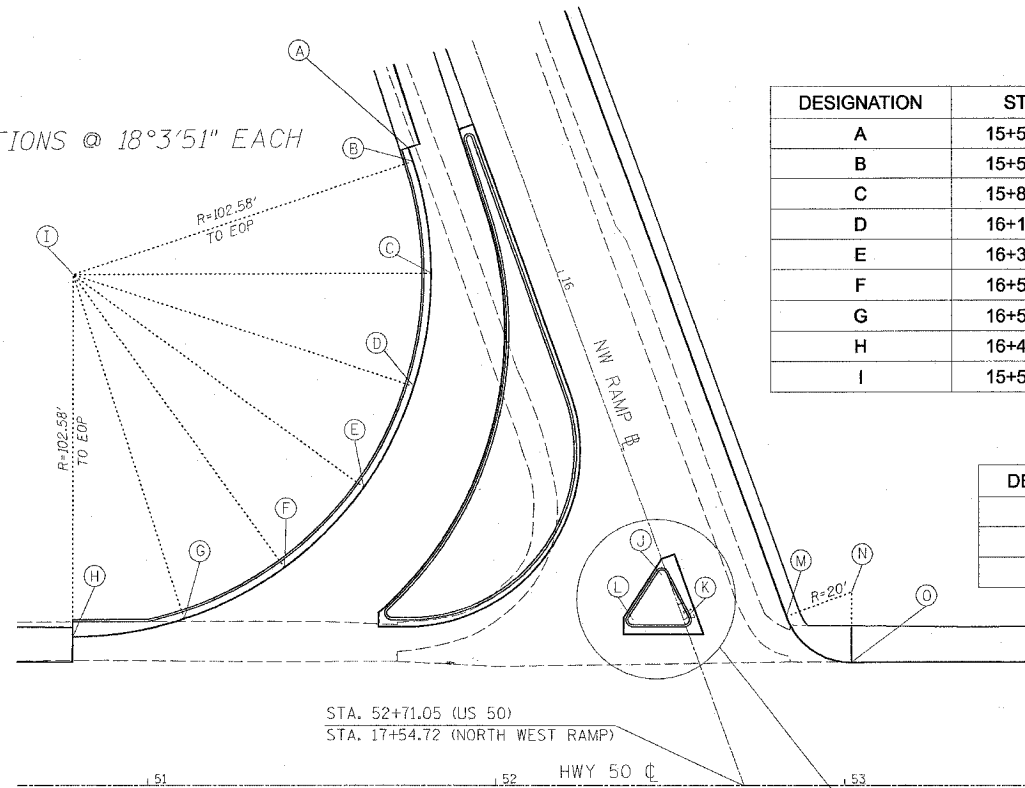
NORTHWEST RAMP LAYOUT (NW QUAD)
