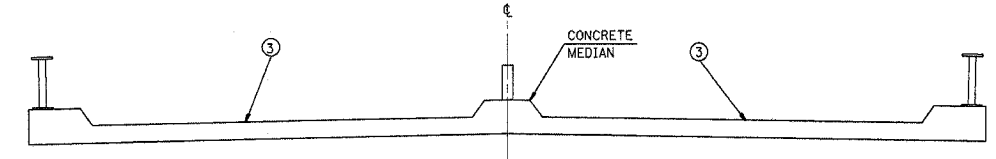
TYPICAL CROSS-SECTION OF ELEVATED ROADWAY TYPICAL EXPRESSWAY CROSS-SECTION NO. 2
