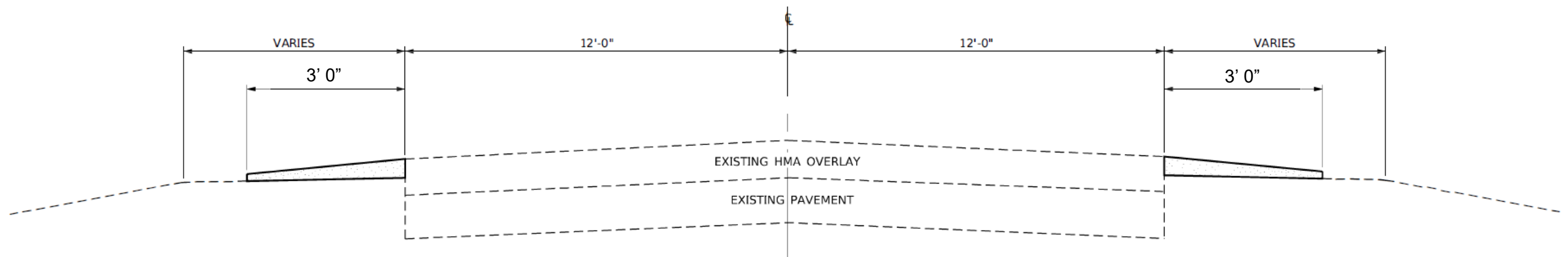
TYPICAL SECTION
