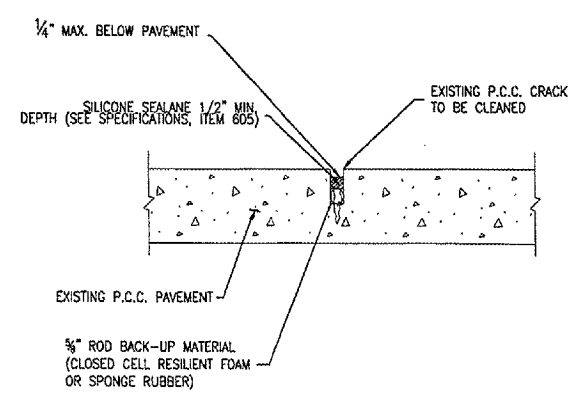
CLEAN AND SEAL CRACKS DETAIL B
