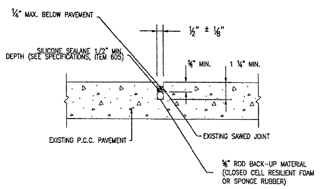
CLEAN AND SEAL JOINTS DETAIL A
