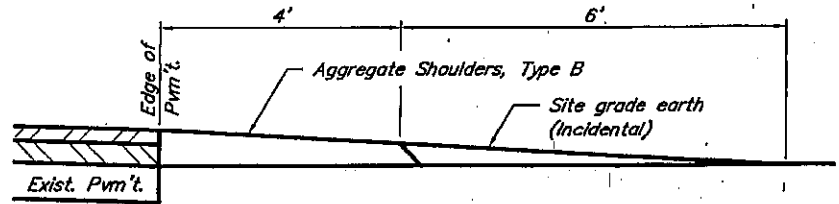
SECTION A-A FIELD ENTRANCE (Est. No. = 40)
