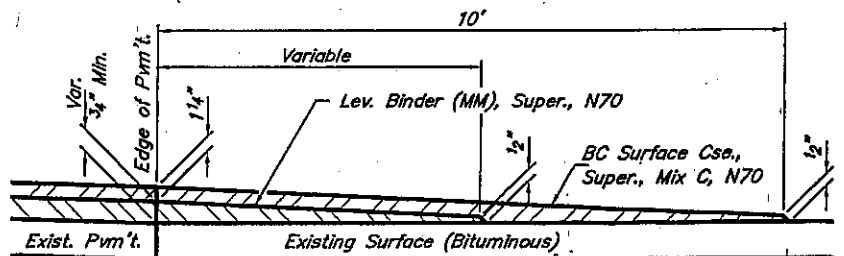
SECTION A-A PRIVATE ENTRANCE - BITUMINOUS (Est. No. = 5)
