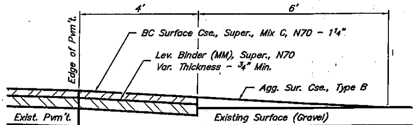
SECTION A-A PRIVATE ENTRANCE - GRAVEL (Est. No. = 55)
