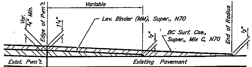
SECTION A-A SIDE ROAD (Est. No. = 12)
