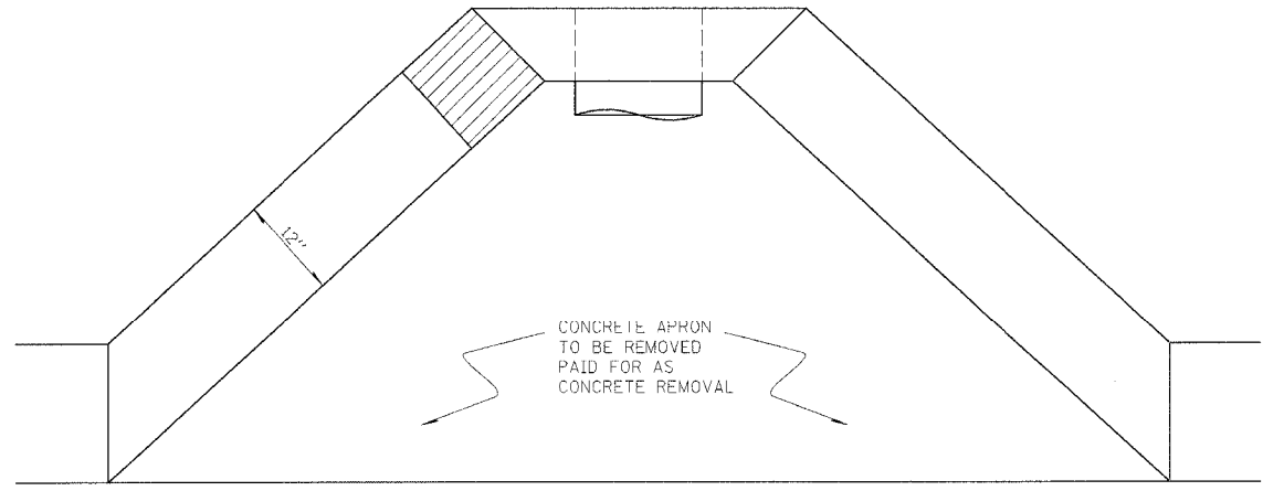
TOP VIEW
