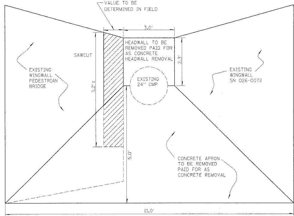
FRONT VIEW REMOVAL
