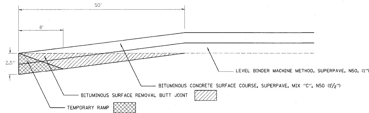
BUTT JOINT DETAIL STATION 1018+21 TO STATION 1018+71 STATION 1050+26 TO STATION 1050+76
