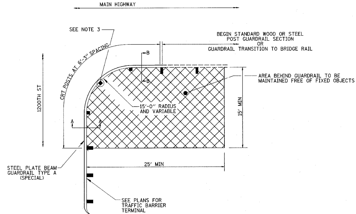
PLAN AT PUBLIC ROAD
