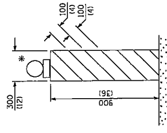
VERTICAL BARRICADE
