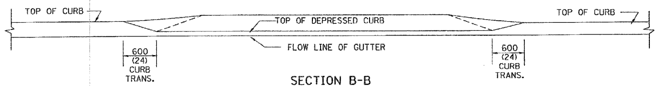
SECTION B-B
