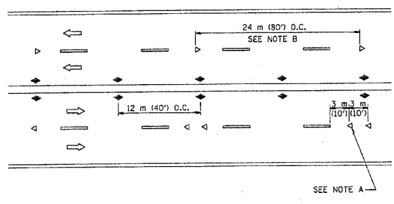
MULTI-LANE/UNDIVIDED
