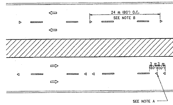
MULTI-LANE/DIVIDED
