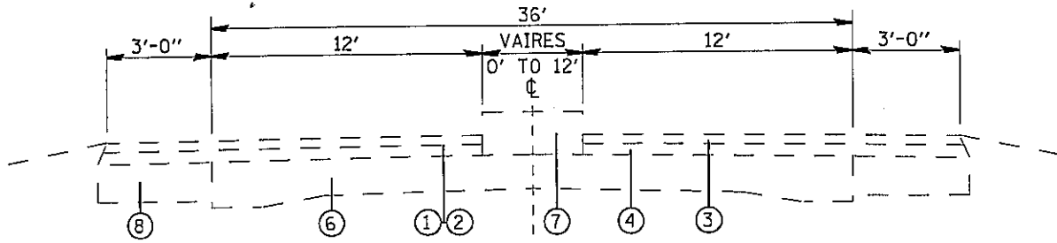
TYPICAL SECTION MM 0.226 TO MM 0.564
