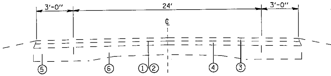
EXISTING TYPICAL SECTION MM 0.000 TO MM 0.128 MM 0.564 TO MM 0.590
