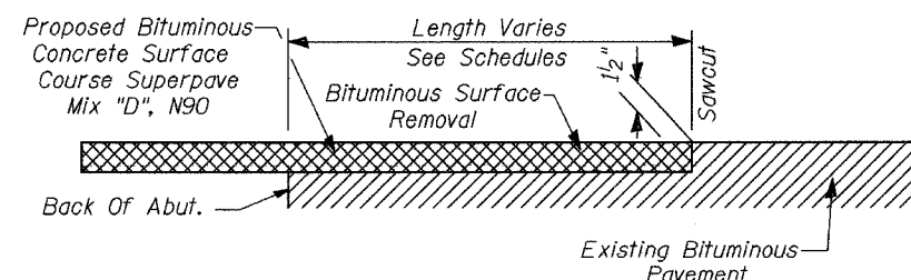
BUTT JOINT DETAIL - SN 101-029 THRU SN 101-0032
