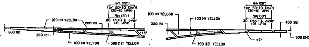
TYPICAL PAVEMENT MARKING FOR FLUSH MEDIAN
