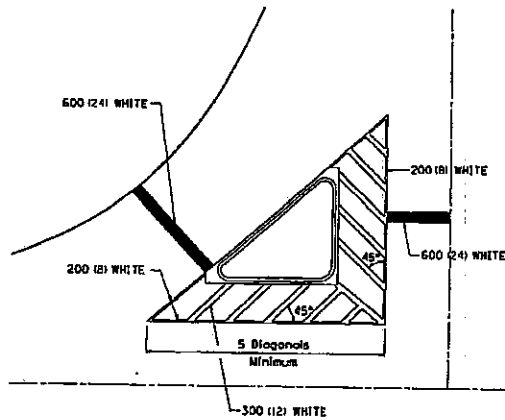
TYPICAL ISLAND OFFSET SHOULDER WIDTH
