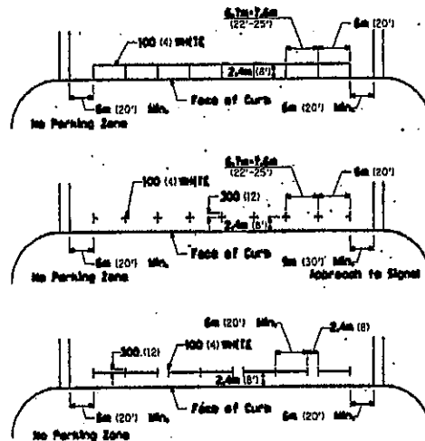
TYPICAL PARKING SPACING
