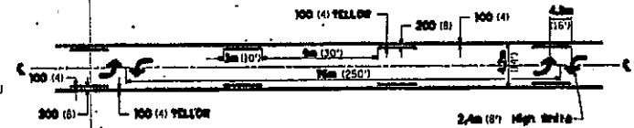
MEDIAN PAVEMENT MARKING
