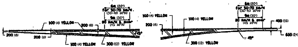
TYPICAL PAVEMENT MARKING FOR FLUSH MEDIAN
