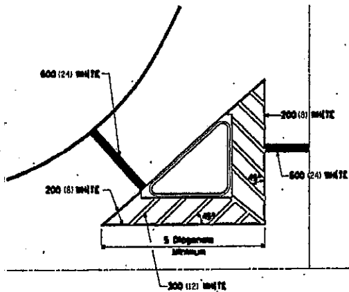
TYPICAL ISLAND OFFSET SHOULDER WIDTH
