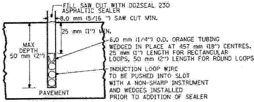
LOOP CROSS SECTION IN PAVEMENT
