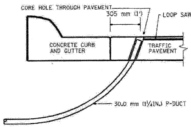
SIDE SECTION LOOP LEAD-IN TRANSITION DETAIL
