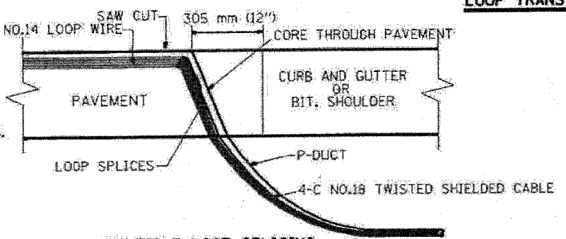
MULTIPLE LOOP SPLICING
