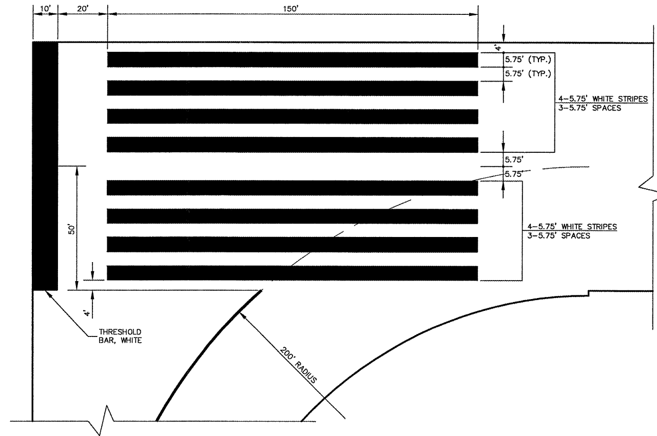
RUNWAY 20 THRESHOLD MARKERS
