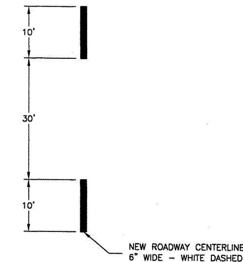
SERVICE ROAD CENTERLINE MARKING N.T.S.
