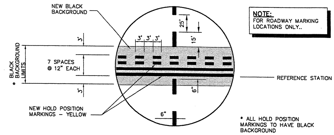
RUNWAY HOLD POSITION MARKING DETAIL N.T.S.
