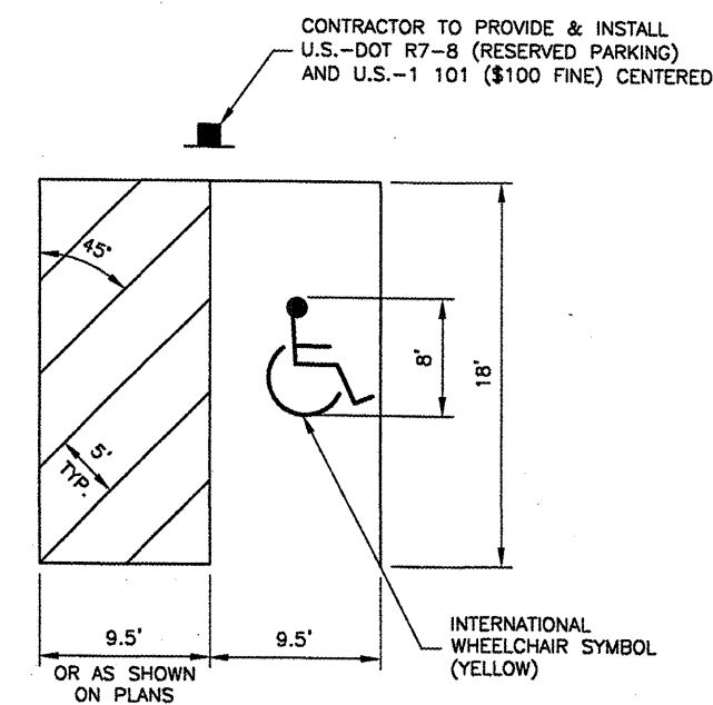
HANDICAP PARKING SPACE N.T.S.
