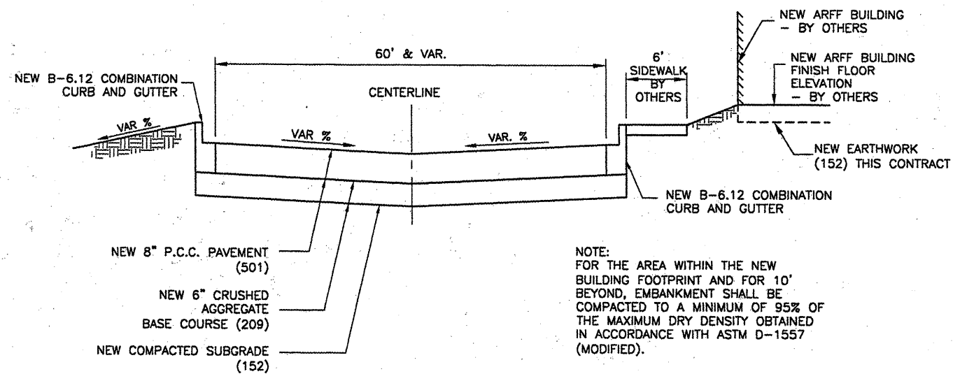
D NEW BUILDING AND PARKING AREA TYPICAL SECTION N.T.S. D
