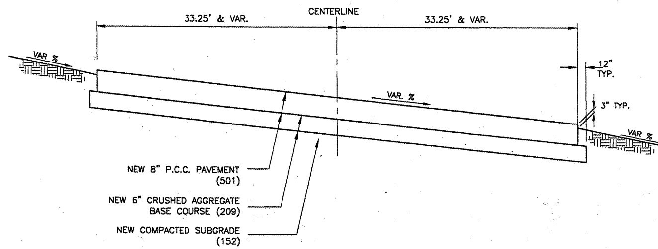
B NEW LAND SIDE/AIR SIDE APRON AND DRIVEWAY TYPICAL SECTION N.T.S. B
