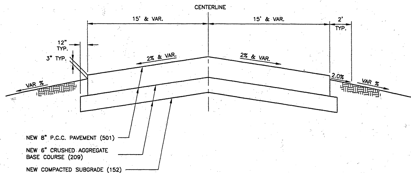
C NEW MAJOR INCIDENT ACCESS/SERVICE ROAD TYPICAL SECTION N.T.S. C
