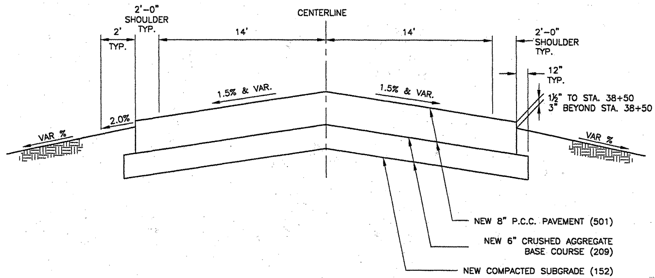
A ARFF RESPONSE ROAD TYPICAL SECTION N.T.S. A
