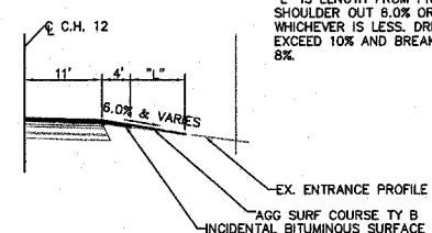
PLAN NOTE: "W" IS WIDTH OF EXISTING ENTRANCE. "L" IS LENGTH FROM PROPOSED EDGE OF SHOULDER OUT 6.0% OR TO EXISTING R.O.W. WHICHEVER IS LESS. DRIVEWAY SLOPE NOT TO EXCEED 10% AND BREAKOVER NOT TO EXCEED 8%.
