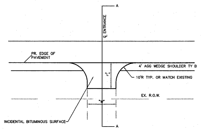
PLAN NOTE: "W" IS WIDTH OF EXISTING ENTRANCE. "L" IS LENGTH FROM PROPOSED EDGE OF SHOULDER OUT 6.0% OR TO EXISTING R.O.W. WHICHEVER IS LESS. DRIVEWAY SLOPE NOT TO EXCEED 10% AND BREAKOVER NOT TO EXCEED 8%.
