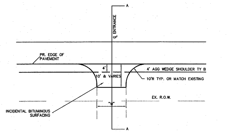
PLAN NOTE: "W" IS WIDTH OF EXISTING ROAD.
