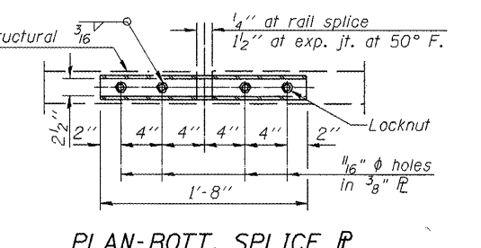
PLAN-BOTT. SPLICE TYPICAL
