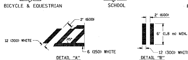
TYPICAL CROSSWALK MARKING
