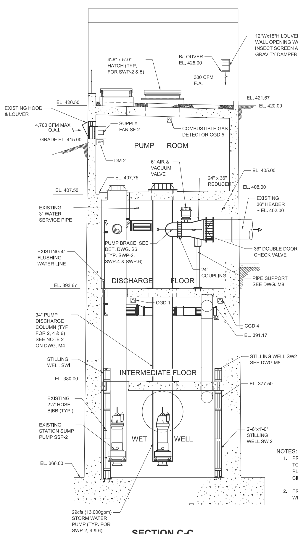
SECTION C-C
