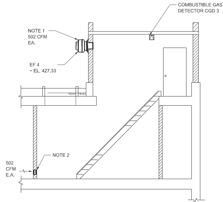
SECTION J-J
