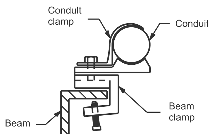
DETAIL C
