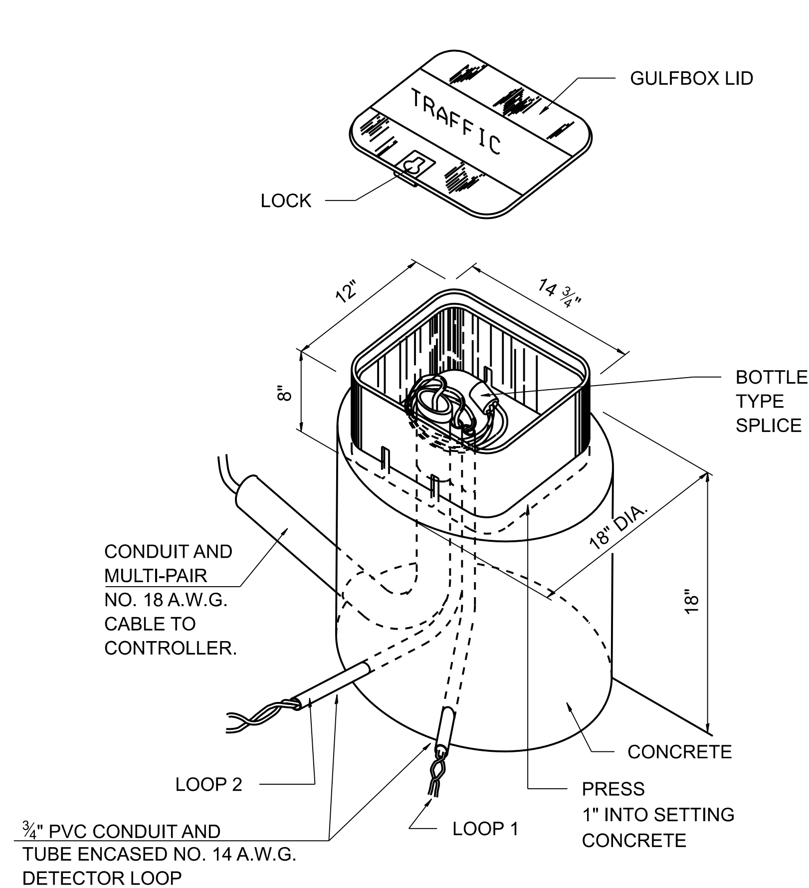
GULFBOX JUNCTION DETAIL (SHOWING CONNECTION OF TUBE-ENCASED DETECTOR LOOP TO MULTI-PAIR LEAD-IN CABLE)
