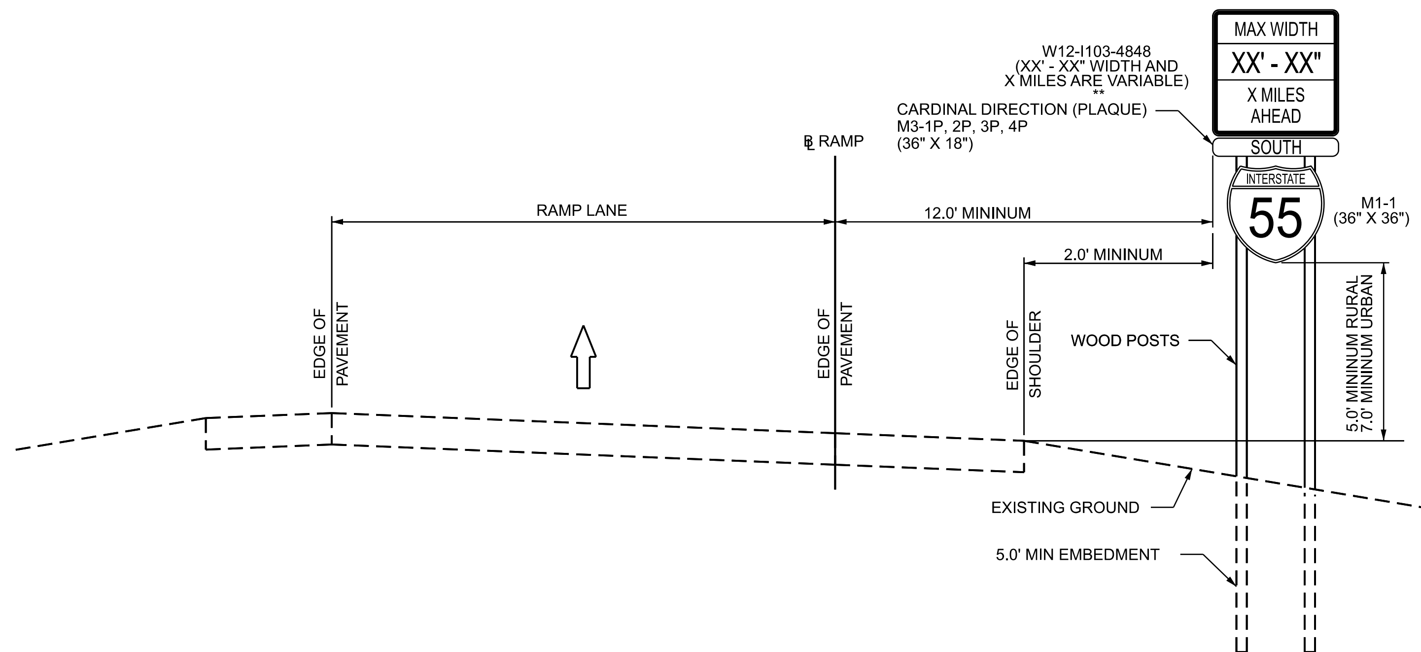
WIDTH RESTRICTION SIGN INTERSTATE AND EXPRESSWAYS RAMP PAVEMENT
