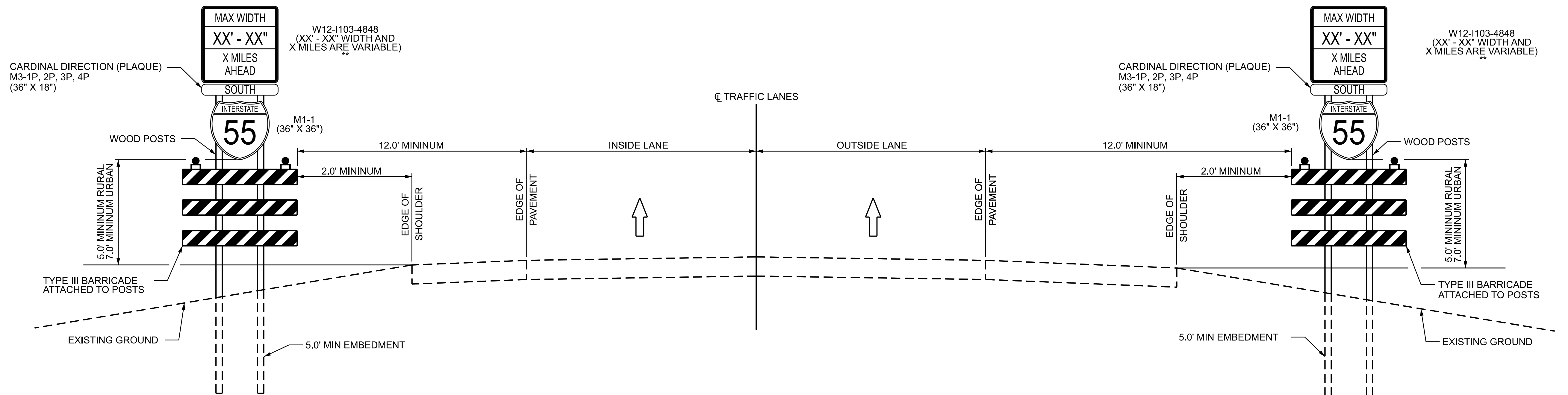
WIDTH RESTRICTION SIGN INTERSTATE AND EXPRESSWAYS MAINLINE PAVEMENT
