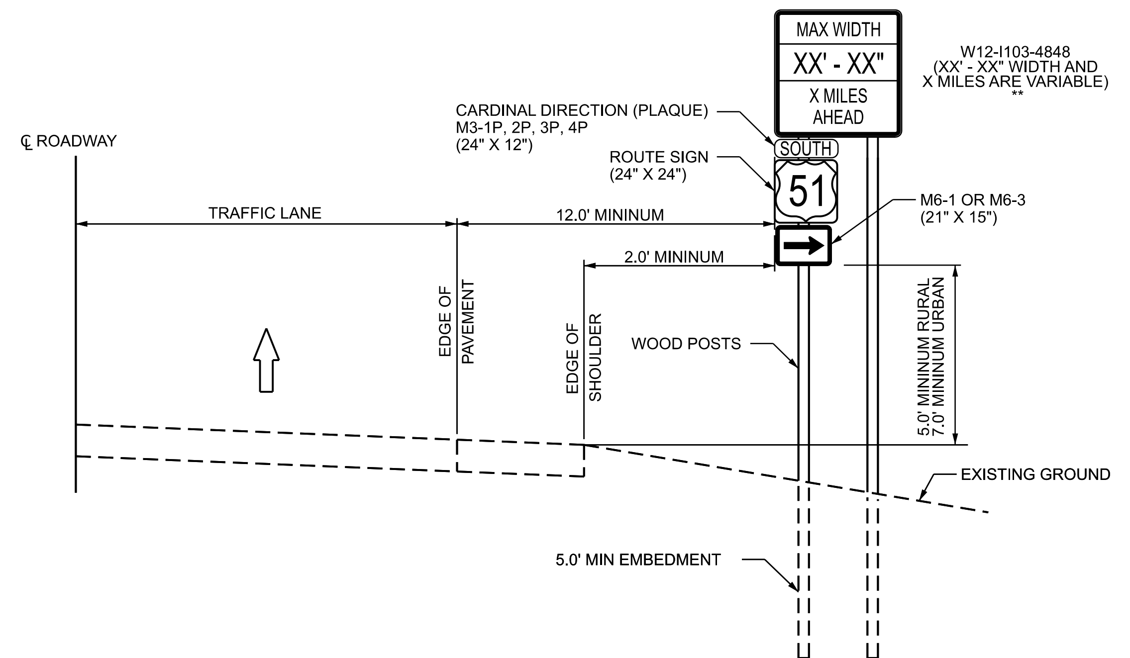
WIDTH RESTRICTION SIGN CONVENTIONAL ROADWAYS
