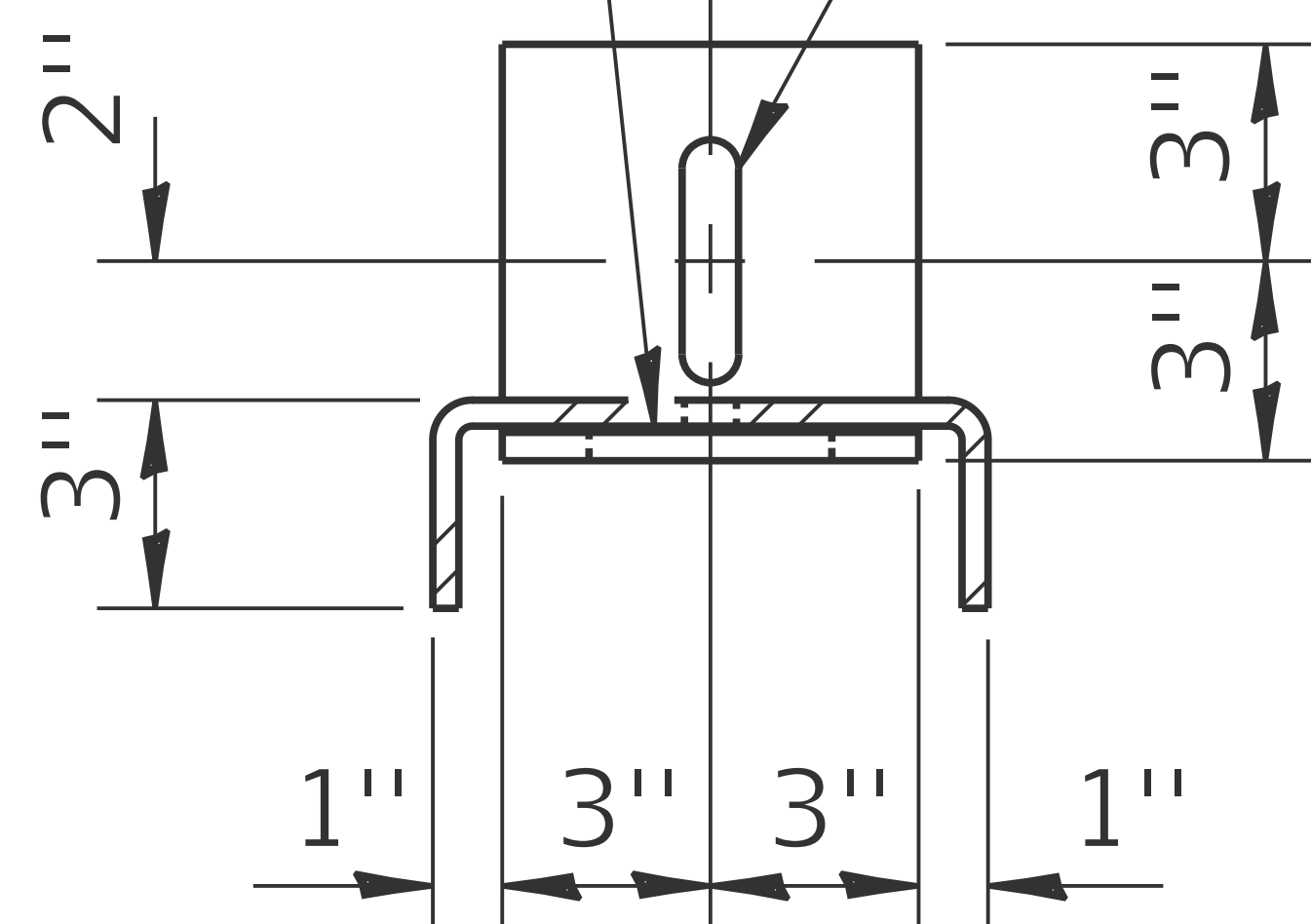
SECTION B-B
