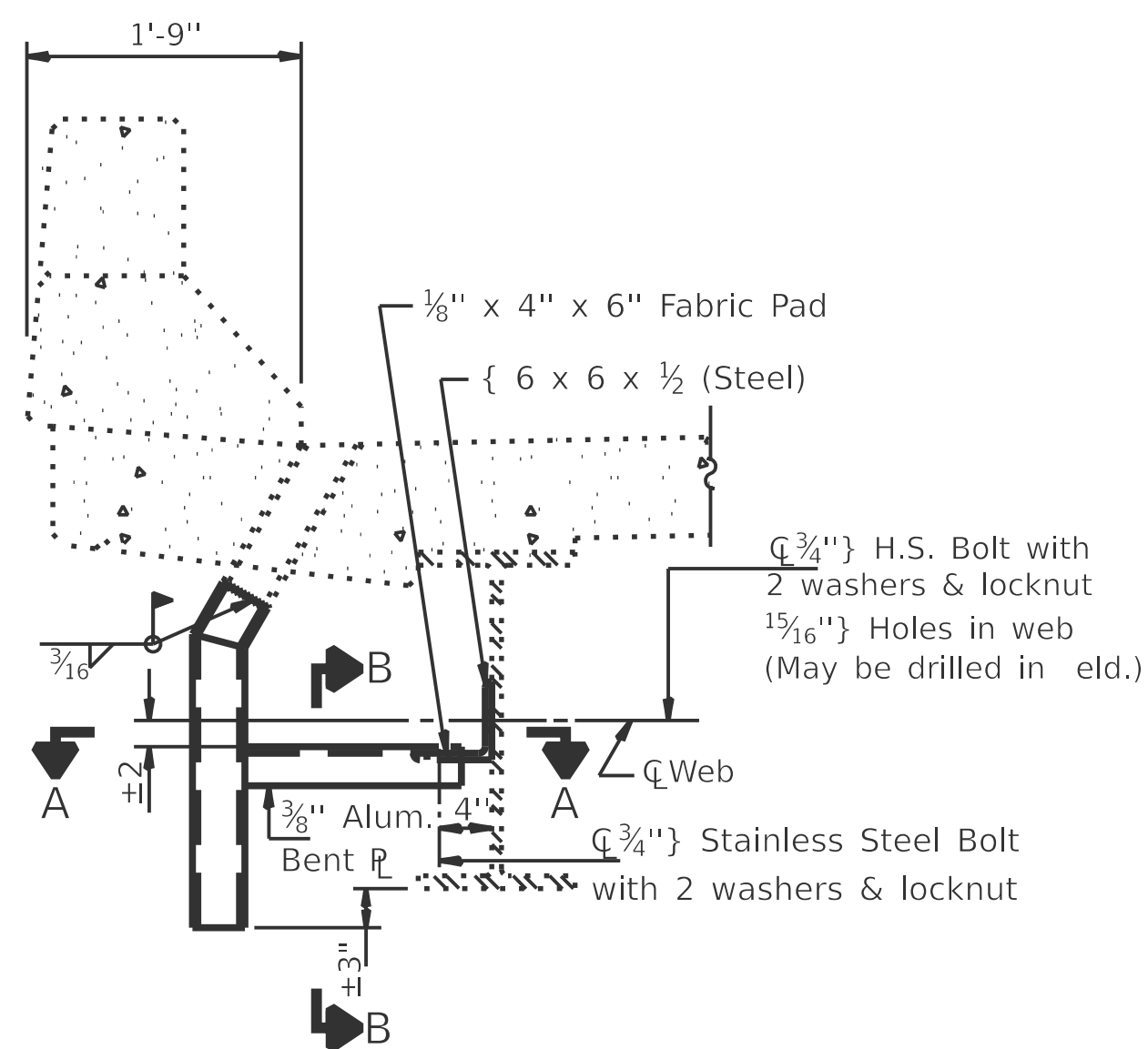
SECTION AT DRAIN
