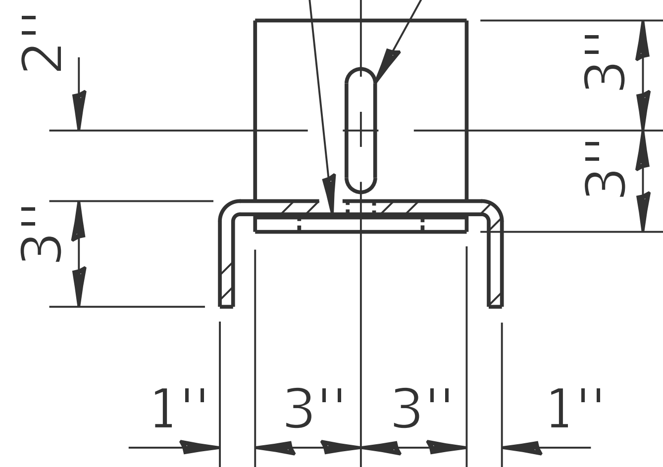
SECTION B-B
