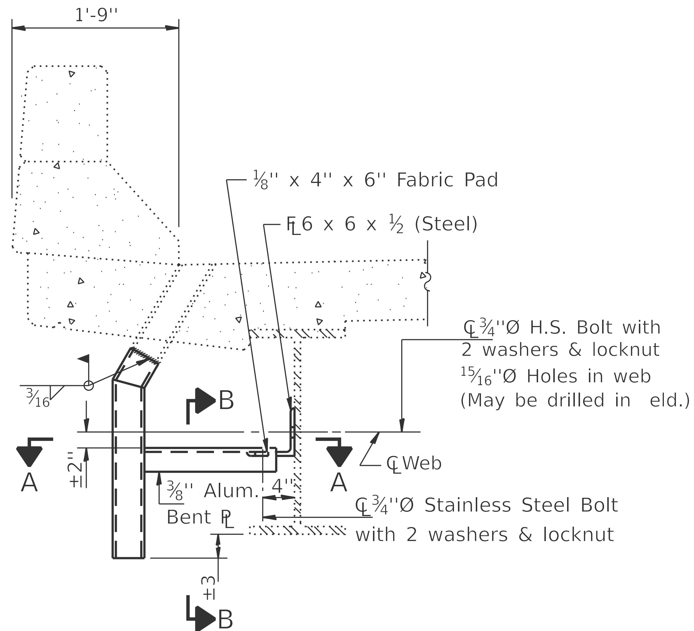
SECTION AT DRAIN
