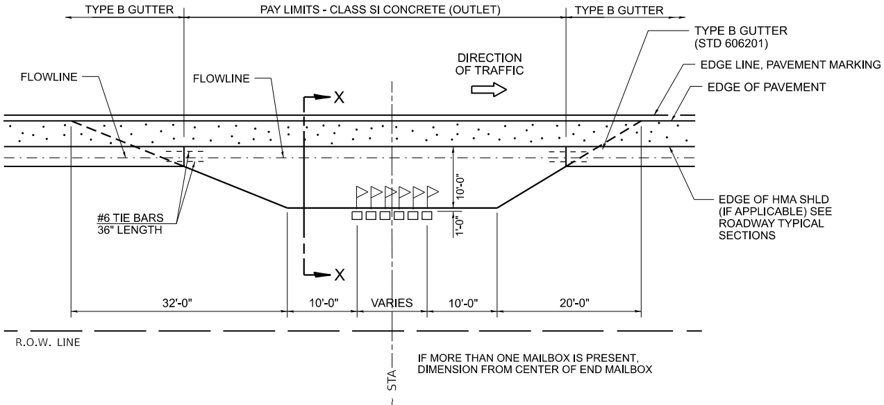
PLAN - RURAL MULTIPLE MAILBOX TURNOUT
