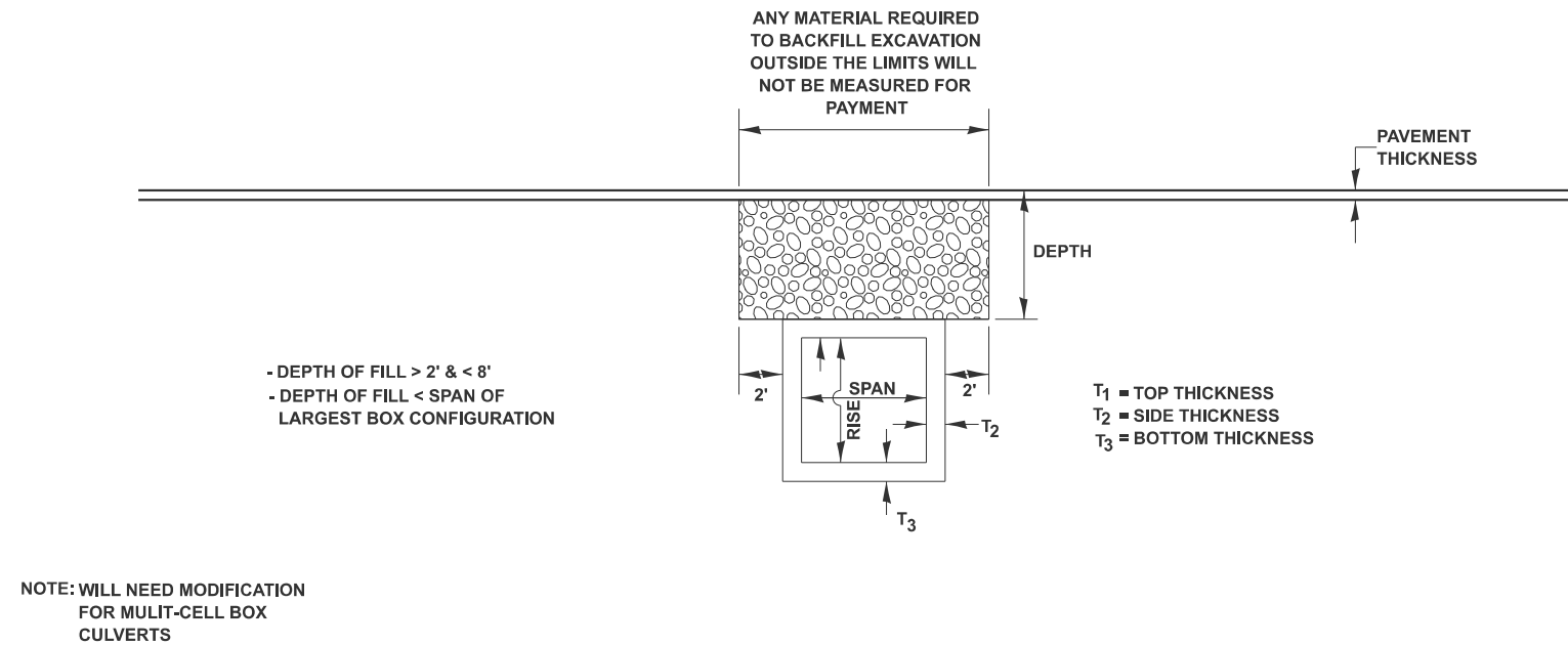
PROFILE GRANULAR BACKFILL DETAIL FOR NEW ALIGNMENTS & CONSTRUCTION
