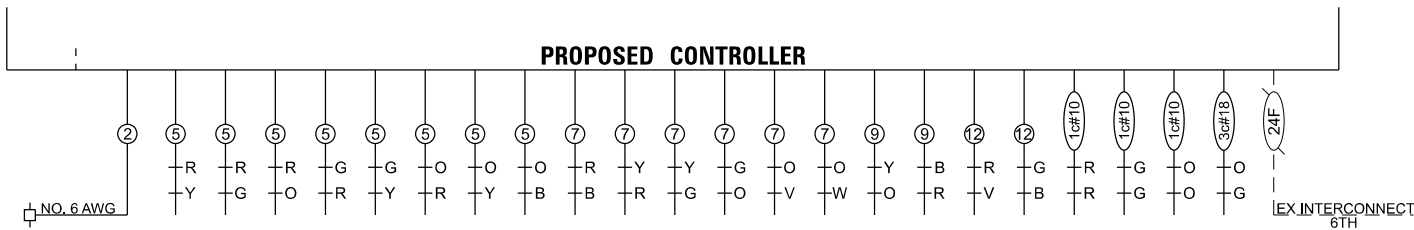
PHASE DESIGNATION DIAGRAM
