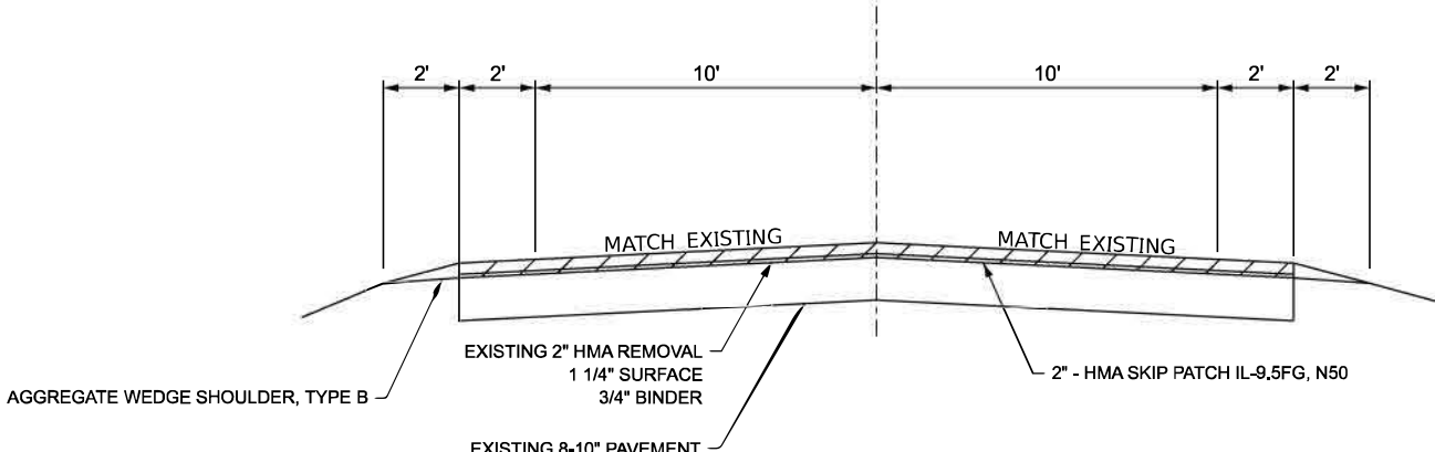
TYPICAL SKIP PATCH @ ATKINSON RD. IL 92 TO PAVEMENT JOINT N. OF RR IN ATKINSON
