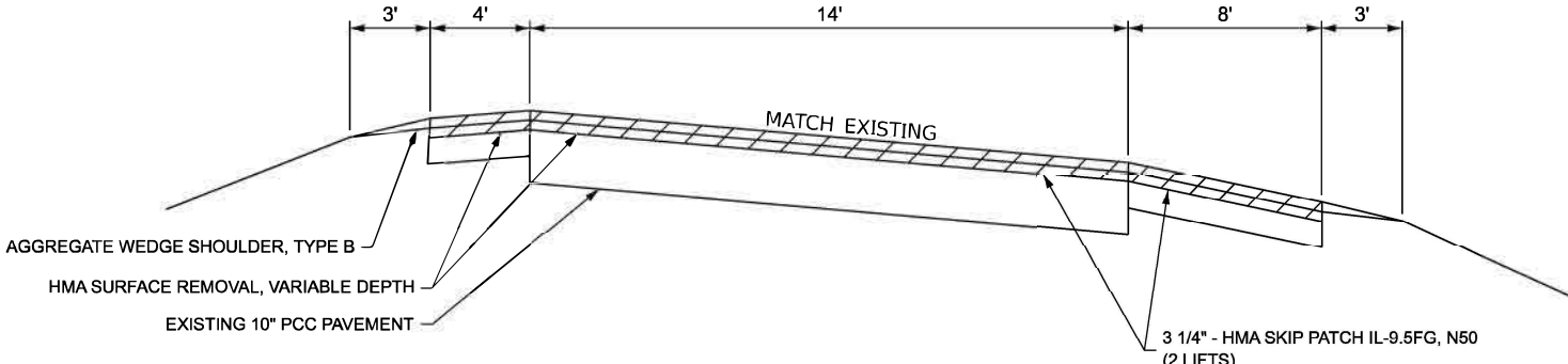
TYPICAL RAMP I-80 @ ATKINSON RD.
