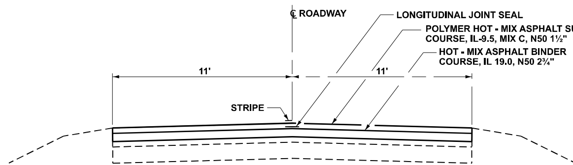
PROPOSED TYPICAL SECTION 2 L. M. 0.79 TO L.M. 1.12 LASALLE COUNTY
