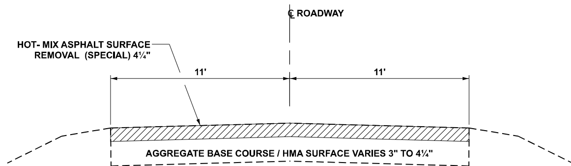
EXISTING TYPICAL SECTION 1 L. M. 0.00 TO L.M. 0.79 BUREAU COUNTY
