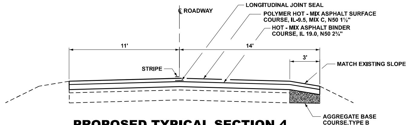
PROPOSED TYPICAL SECTION 4 L. M. 1.12 TO L.M. 1.25 LASALLE COUNTY
