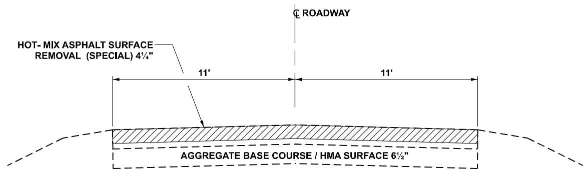
EXISTING TYPICAL SECTION 5 L. M. 1.25 TO L.M. 1.355 LASALLE COUNTY
