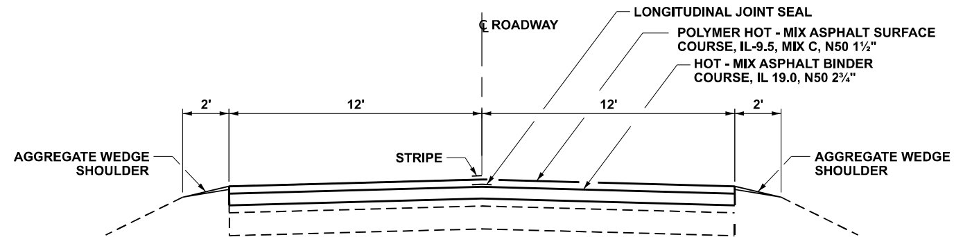
PROPOSED TYPICAL SECTION 5 L. M. 1.25 TO L.M. 1.355 LASALLE COUNTY
