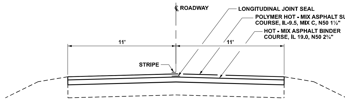
PROPOSED TYPICAL SECTION 1 L. M. 0.00 TO L.M. 0.79 BUREAU COUNTY
