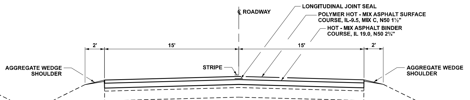
PROPOSED SECTION 6 L. M. 1.355 TO L.M. 1.36 LASALLE COUNTY
