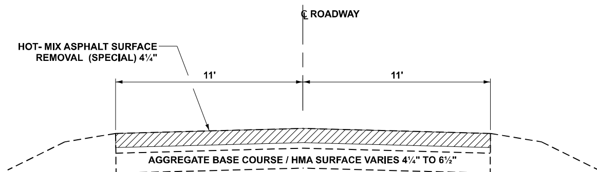
EXISTING TYPICAL SECTION 2 L. M. 0.79 TO L.M. 1.12 LASALLE COUNTY
