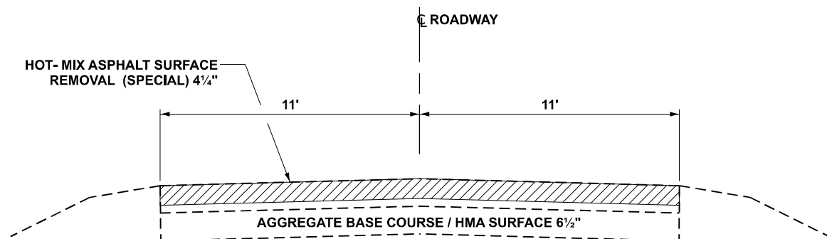
EXISTING TYPICAL SECTION 3 L. M. 1.12 TO L.M. 1.25 LASALLE COUNTY
