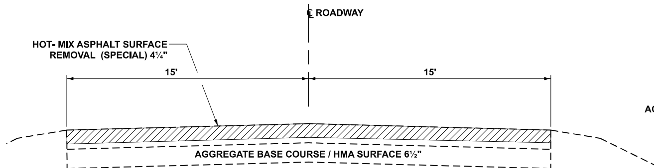
EXISTING TYPICAL SECTION 6 L. M. 1.355 TO L.M. 1.36 LASALLE COUNTY
