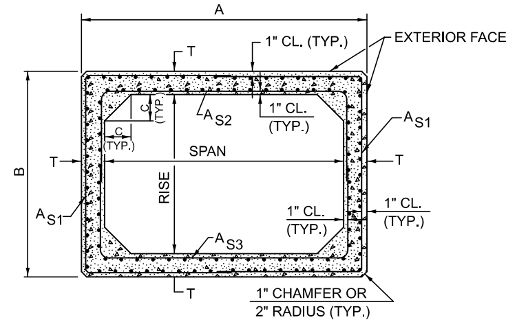
CROSS SECTION
