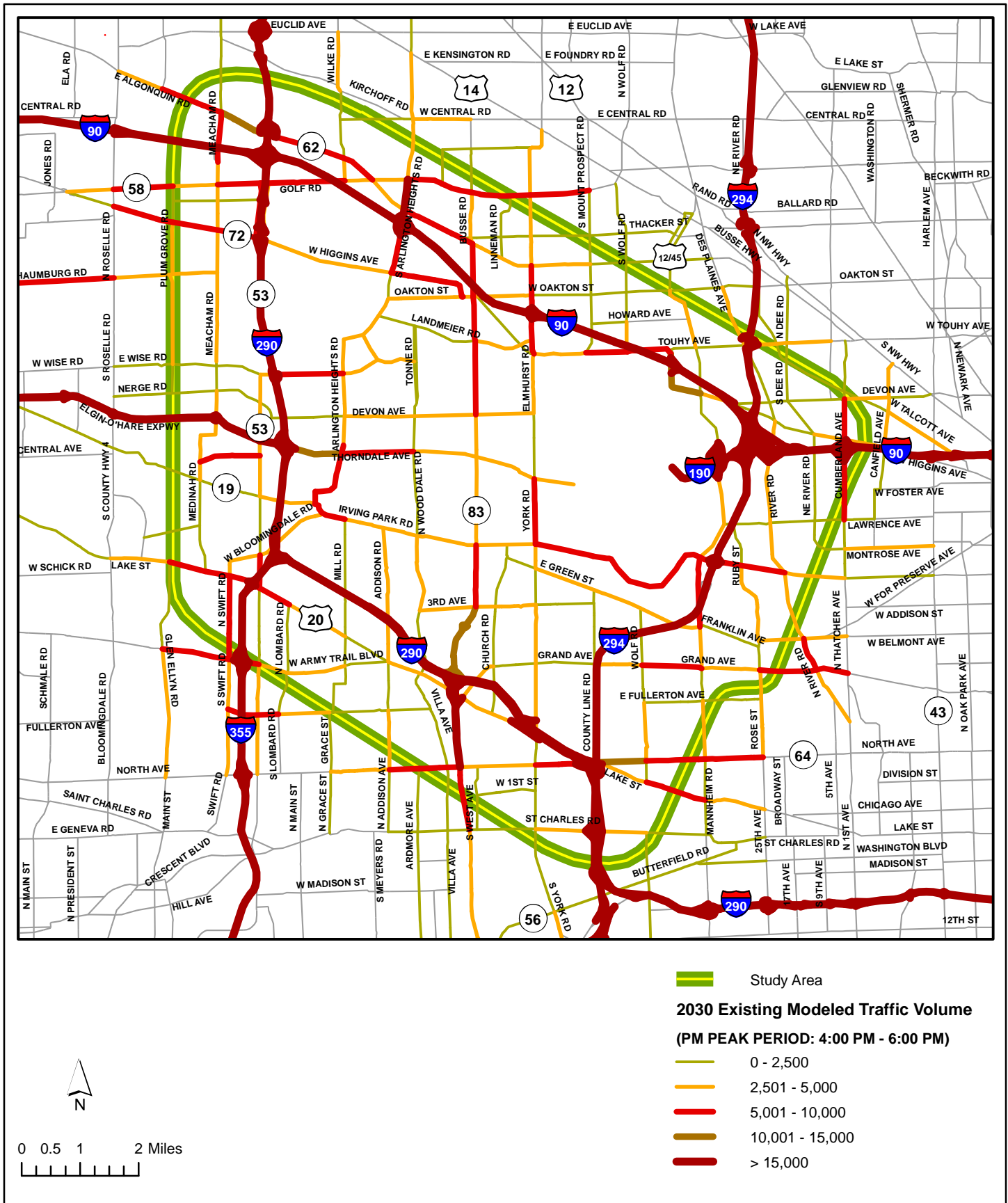
Elgin O'Hare - West Bypass 2030 P.M. Peak Period Modeled Traffic Volume Exhibit 4-5
