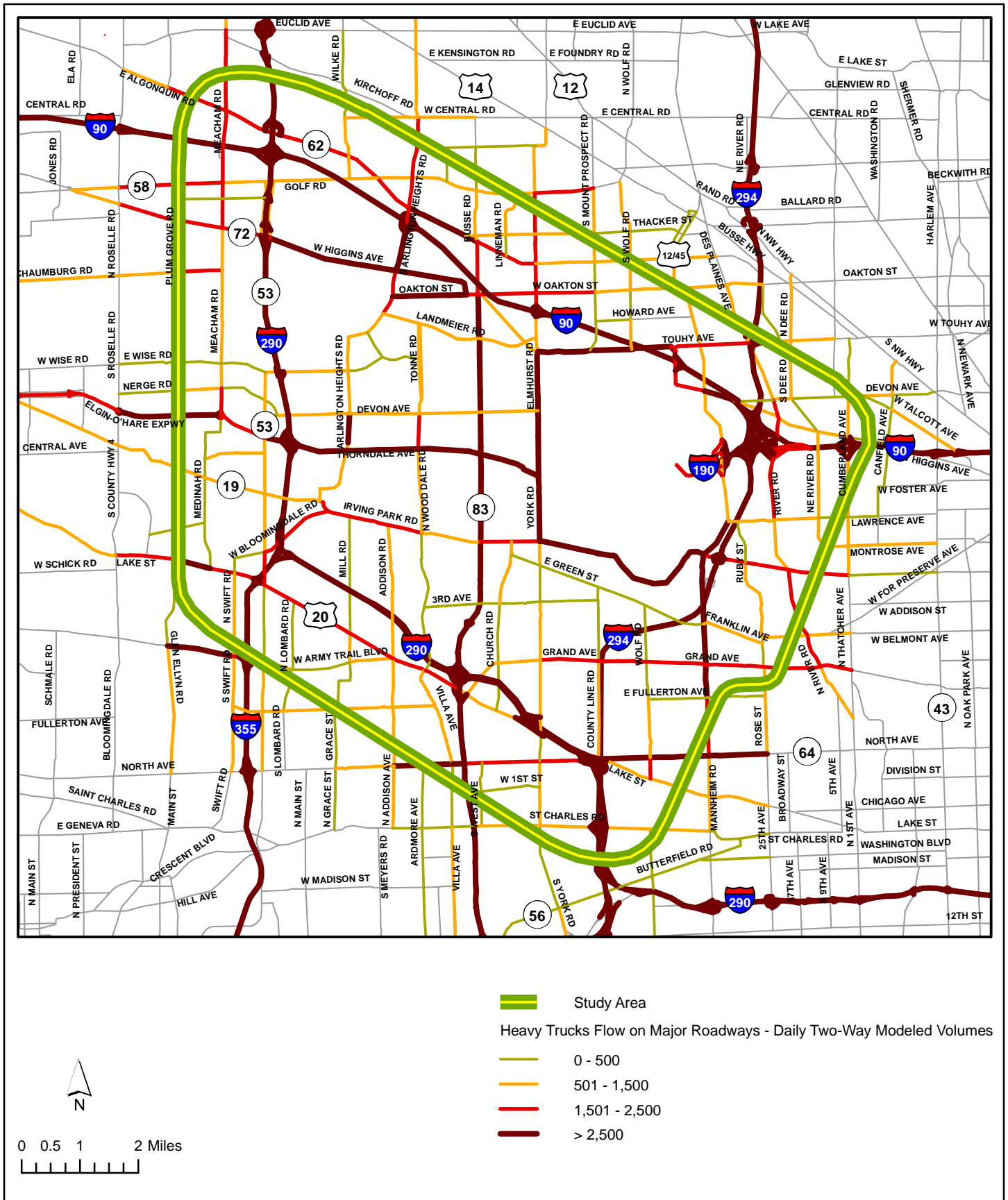
Elgin O'Hare - West Bypass 2007 Daily Modeled Heavy Truck Volume Exhibit 3-8
