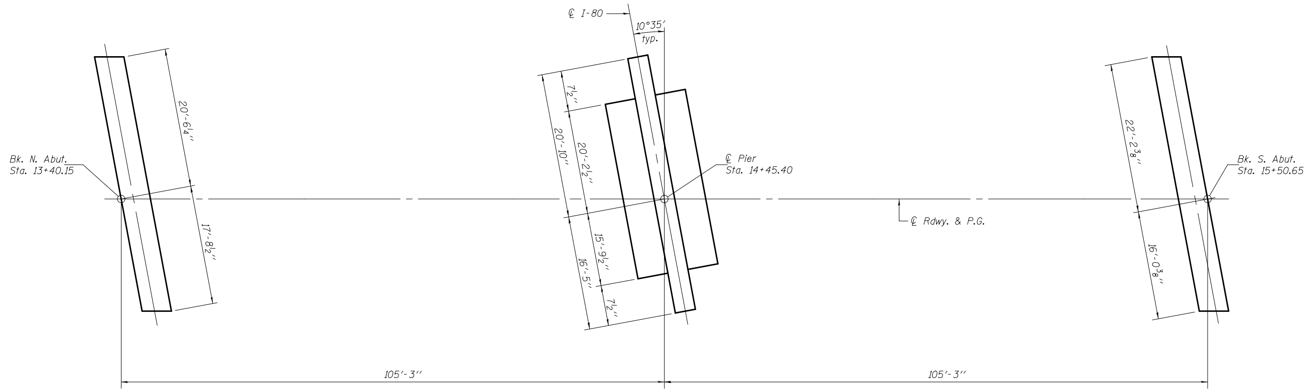
FOOTING LAYOUT
