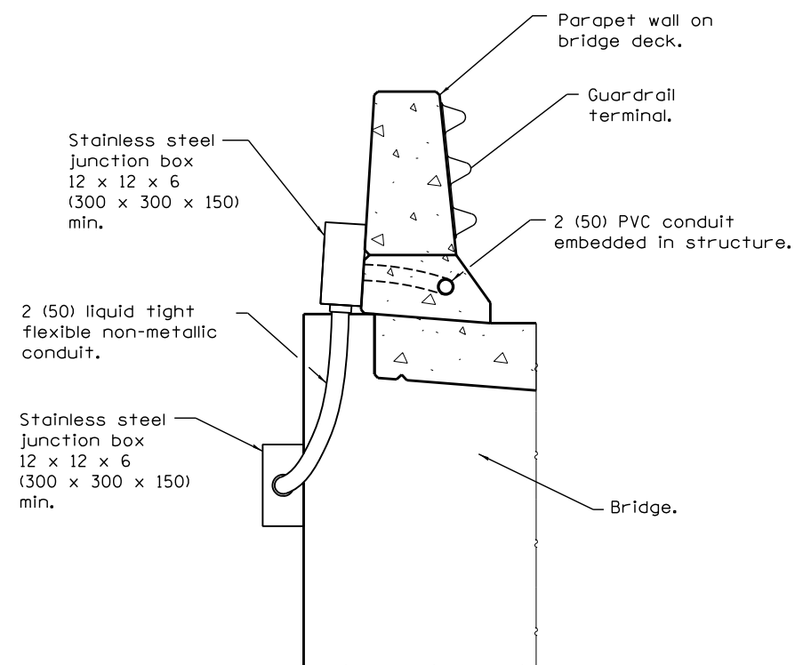
VIEW B-B
