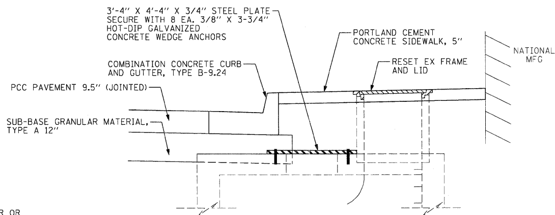
A-A (PROPOSED)
