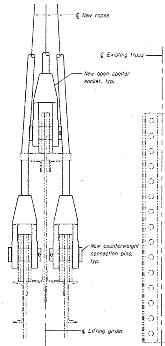
SECTION B-B
