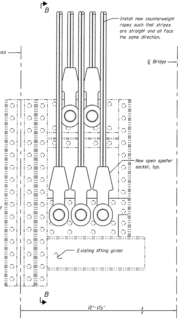
CONNECTION AT LIFT GIRDER (4 Locations)
