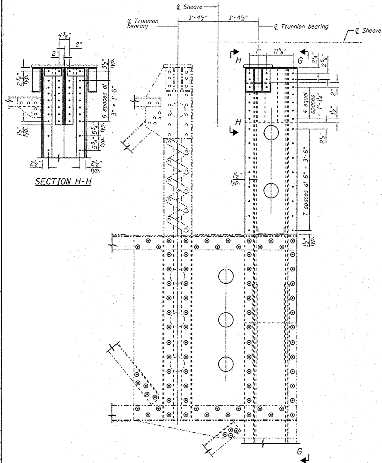
BOLT LEGEND ELEVATION - NEW VERTICAL TOWER POST BOLT LAYOUT DETAIL
