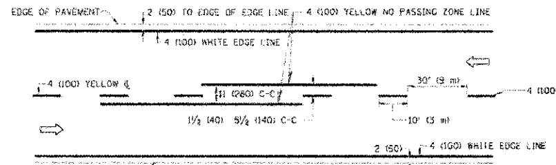
2-LANE ROADWAY
