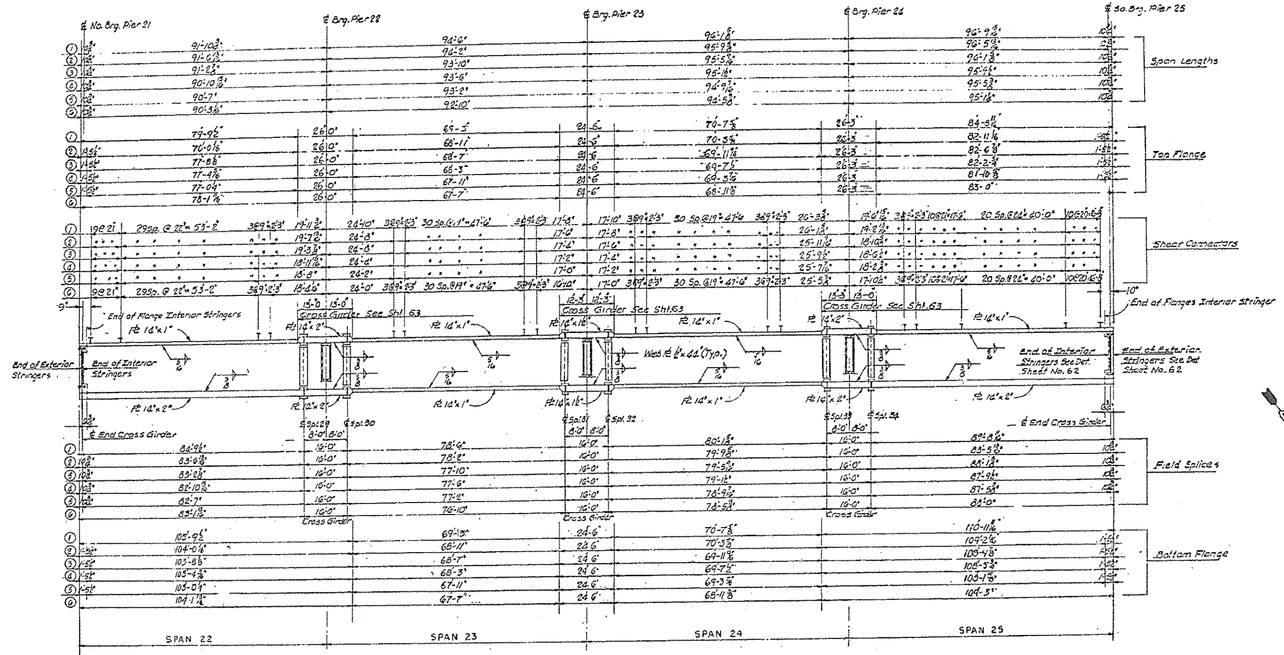
GIRDER ELEVATION
