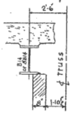
SECTION A-A scale 3/4" = 1'-0"
