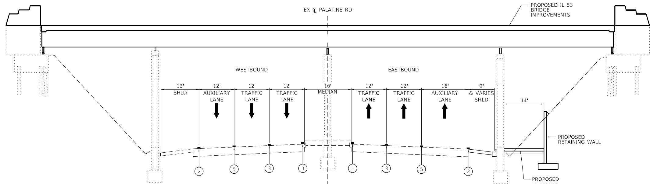
PALATINE ROAD AT IL 53 WINTER SHUTDOWN STA. 818+06.10 TO STA. 819+92.74
