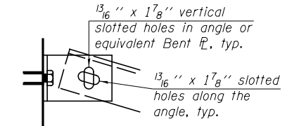
DETAIL B
