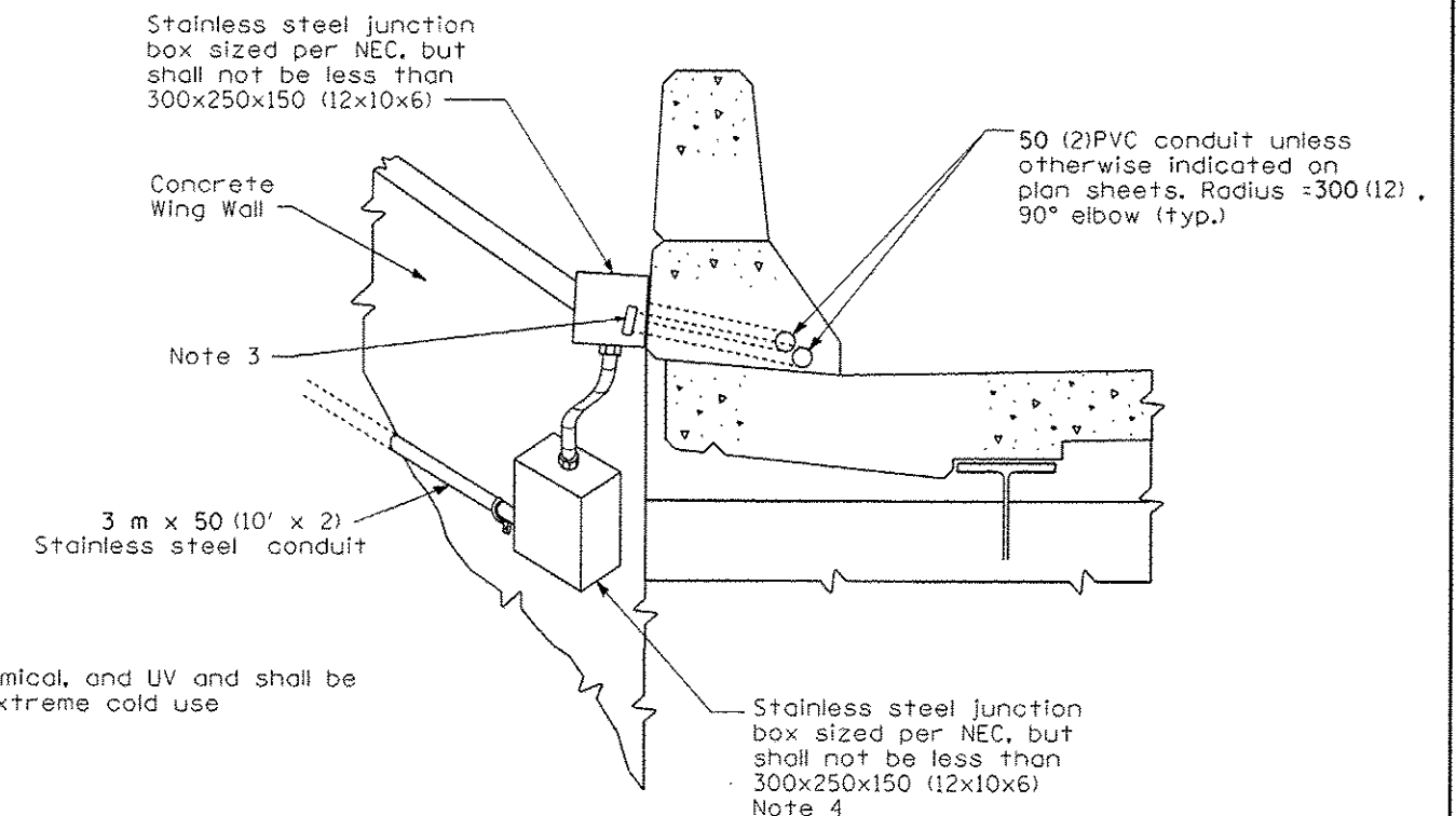
SECTION B-B DETAIL \"B\"
