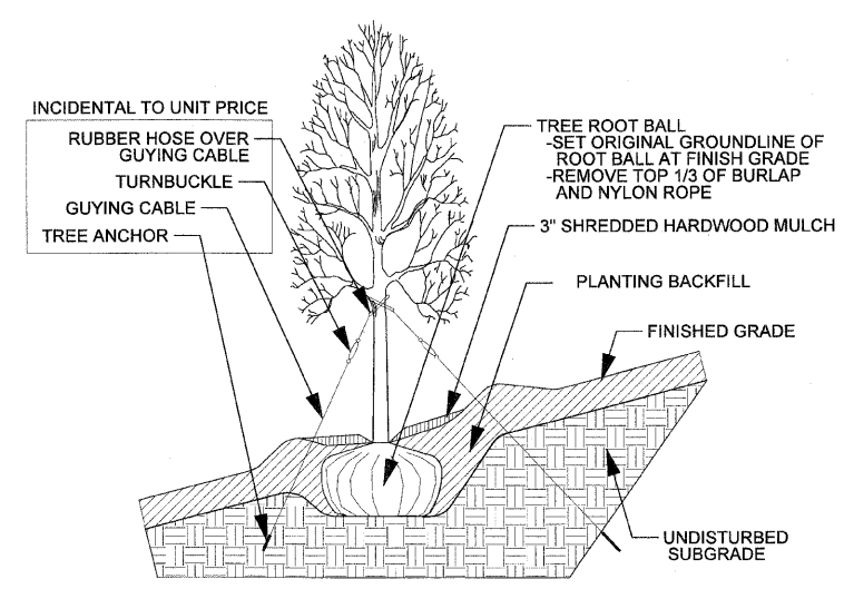
5 TREE PLANTING ON SLOPE DETAIL No Scale
